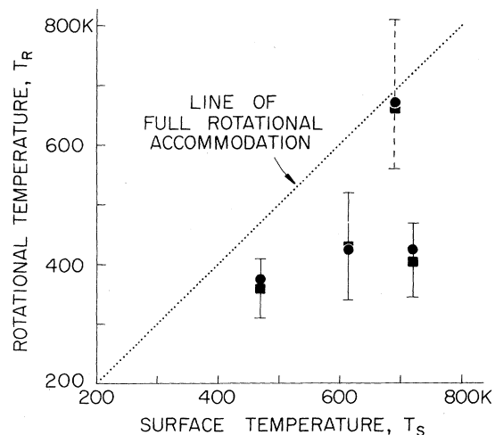
FIG. 3. Plot of T_R vs T_S : full squares obtained from bandhead ratios, \epsilon(T_R) , and full circles obtained from best fit to line features. The solid error bars refer to scattering of NO from Ag(111), the dashed error bar to stainless steel.
