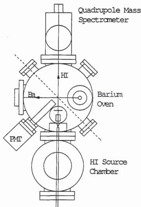
FIG. 1. A schematic diagram of the crossed-beam reaction apparatus employed for the measurement of D_0^0(\text{BaI}) . "Effusive" Ba( ^1S_0 ) and supersonic HI( X^1\Sigma^+ ) beams intersect at 90° geometry to produce BaI product molecules under well-defined, single-collision conditions.
