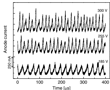
Fig. 6 Oscillograms of discharge current. Xenon flow rate is 0.17 mg/s.
