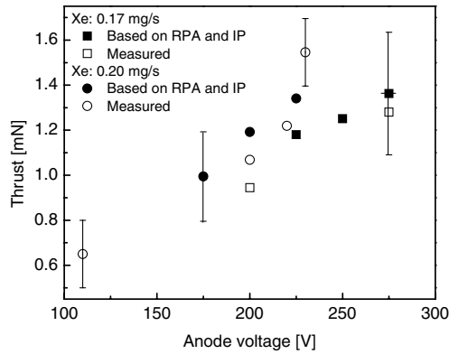
Fig. 14 Thrust as a function of the discharge voltage. Note: error bars are based on estimated 20% error in ion current and 0.15 mN uncertainty associated with direct-thrust measurements.
