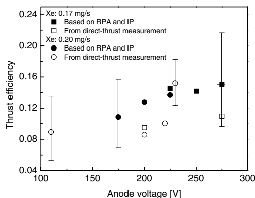
Fig. 15 Anode thrust efficiency as a function of the discharge voltage.
