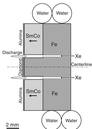
Fig. 1 Schematic of the micro-Hall thruster.
