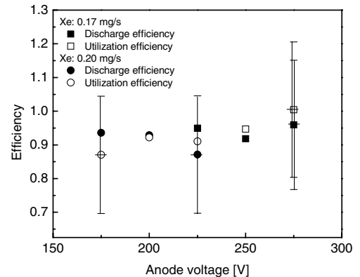
Fig. 11 Discharge and utilization efficiencies as a function of the discharge voltage. The effect of multiply charged ions is neglected. Note: error bars are based on the estimated 20% error in ion current.
