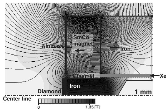
Fig. 3 Simulations of the micro-Hall thruster vacuum magnetic field.
