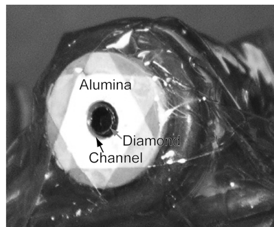
Fig. 2 Photograph of the micro-Hall thruster.
