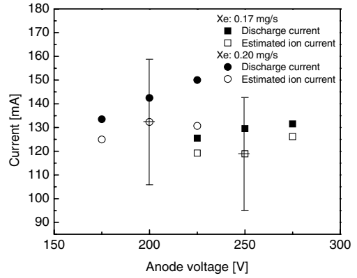
Fig. 10 Discharge and ion current as a function of the discharge voltage. Note: error bars (shown only on maximum or minimum points) are based on the estimated 20% error in ion current.
