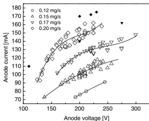
Fig. 5 Voltage-current characteristics. Note: solid symbols are for values observed during direct-thrust measurements.
