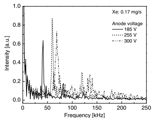
Fig. 7 Low-frequency spectral analysis of the discharge current.
