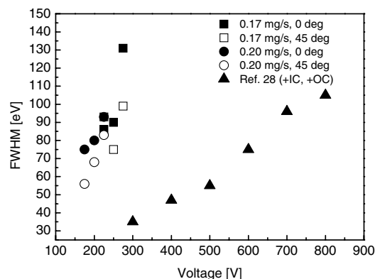
Fig. 13 Width of the ion energy distribution (primary peak) as a function of discharge voltage. Also shown are the widths measured in a 5 kW thruster [28].
