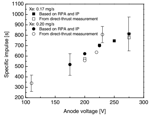
Fig. 16 Anode specific impulse as a function of the discharge voltage.
