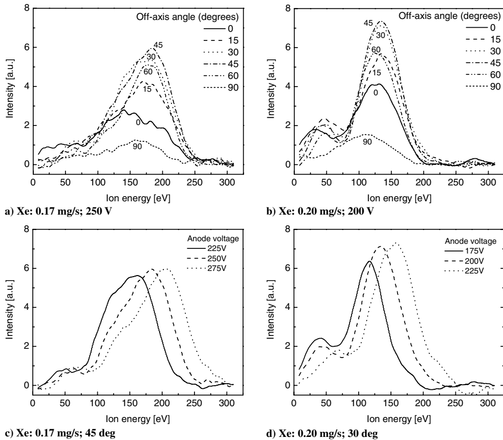
Fig. 12 Examples of ion energy distributions: a–b) angle dependence on xenon flow rate; c–d) anode voltage dependence on Xe flow rate. Note: energy is shifted from the observed value based on the ground potential by a plasma potential of 20 V.
