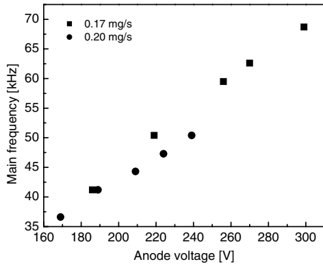
Fig. 8 Mean fundamental breathing mode frequency as a function of the discharge voltage.
