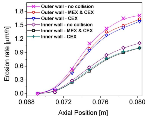
Fig. 10. Effect of particle collisions on the erosion rate of the outer wall.
