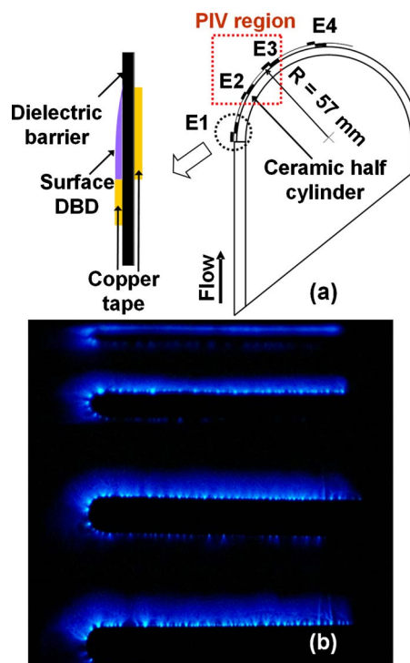
FIG. 1. (Color online) (a) Schematic of DBD actuator and bluff body and (b) rf DBD produced by the actuators viewed at 90° such that E1 is located at the bottom.
