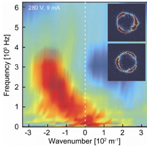
FIG. 3. (Color online) Wave dispersion map for the 280 V case derived from the azimuthally spaced electrostatic probes. The inset shows two images from the high speed emission studies.
