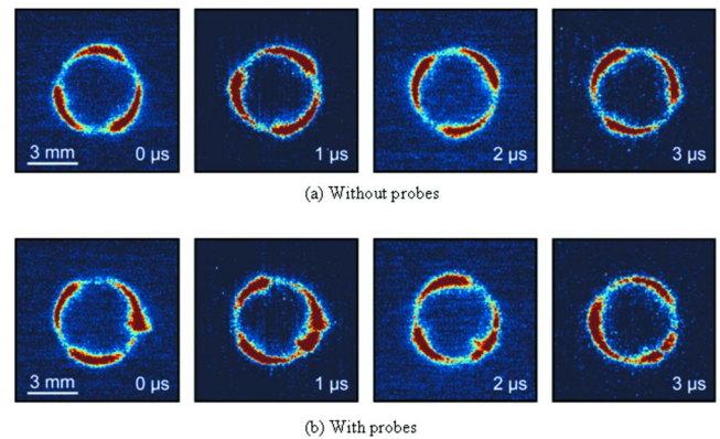
FIG. 2. (Color online) Images taken of the magnetized argon plasma (277 V and 9.3 mA). The gate width of the intensifiers is 0.75 \mu s. (a) Without the probes in position. (b) With the probes in position.
