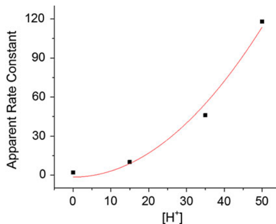
Fig. 5. Apparent rates of acid-induced chlorophyll a demetallation at different concentrations of hydrogen ion. The red line is the best fit to a quadratic dependence on [\text{H}^+] .
