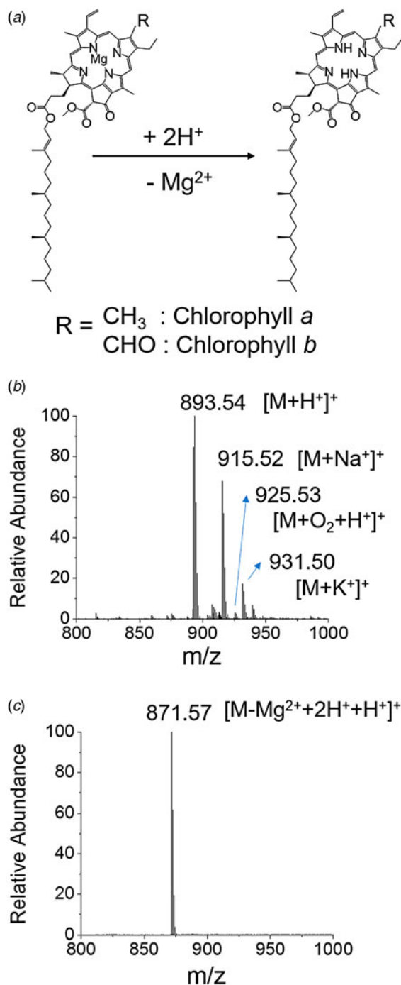
Fig. 1. (a) Reaction scheme of acid-induced demetallation of chlorophyll to form phaeophytin. Mass spectra of chlorophyll a , (b) before and (c) after adding 35 mM HCl.
