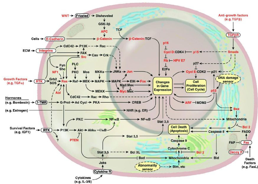
Figure 3.9. The wiring diagram of the growth signaling circuitry of the mammalian cell [16].
