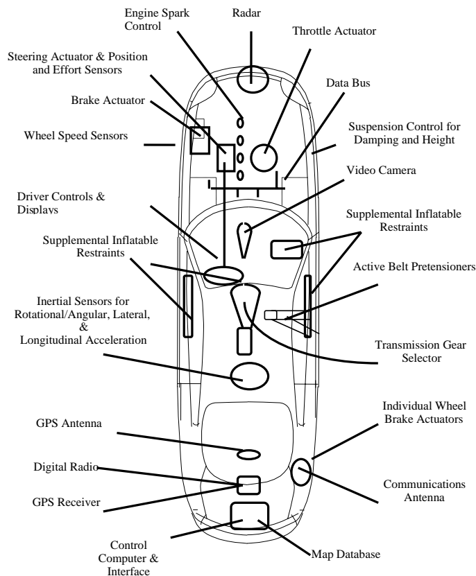
Figure 3.3. Major future components for basic automotive vehicle functions [37].
