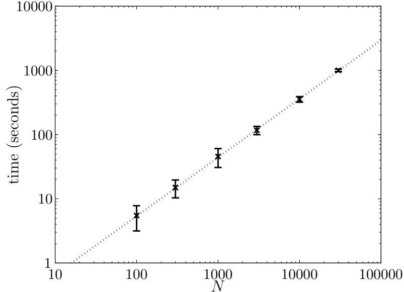
Figure 7: Average prox-average execution times for a family of networks on 8 cores. Error bars show 95% confidence bounds. The dotted line shows the least-squares fit to the data on a log-log scale, resulting in an exponent of 1.03.
