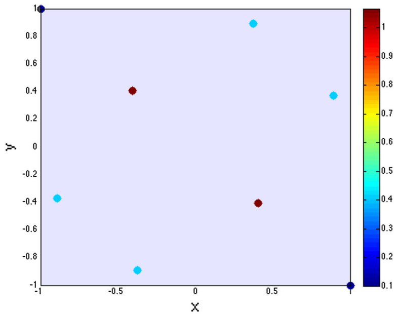
(b) More efficient quadrature obtained with different r .
