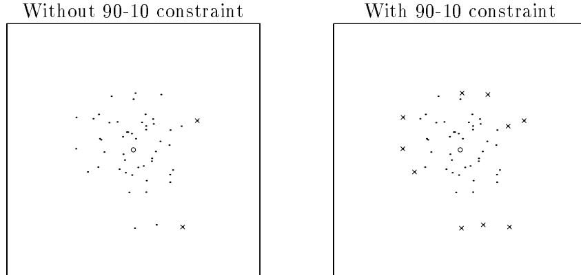
Figure 2: A D -optimal experiment design involving 50 test vectors in \mathbf{R}^2 , with and without the 90-10 constraint. The circle is the origin; the dots are the test vectors that are not used in the experiment ( i.e. , have a weight \lambda_i = 0 ); the crosses are the test vectors that are used ( i.e. , have a weight \lambda_i > 0 ). Without the 90-10 constraint, the optimal design allocates all measurements to only two test vectors. With the constraint, the measurements are spread over ten vectors, with no more than 90% of the measurements allocated to any group of five vectors. See also Figure 3.
