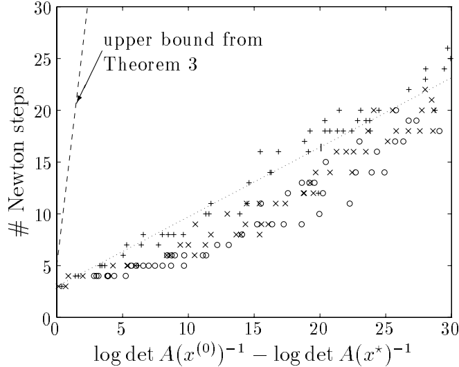
Figure 5: Number of Newton iterations to minimize \log \det A(x)^{-1} versus \log \det A(x^{(0)})^{-1} - \log \det A(x^*)^{-1} (with \delta = 2.33 \cdot 10^{-10} , i.e., \log_2 \log_2(1/\delta) = 5 ). Random matrix completion problems of three sizes ('+': m = 20 ; l = 20 , 'x': m = 20 , l = 100 , 'o': m = 50 , l = 100 ). The dotted line is a least-squares fit of the data and is given by 3 + 0.67(\log \det A(x^{(0)})^{-1} - \log \det A(x^*)^{-1}) . The dashed line is the upper bound of Theorem 3 ( 5 + 11(\log \det A(x^{(0)})^{-1} - \log \det A(x^*)^{-1}) ).
