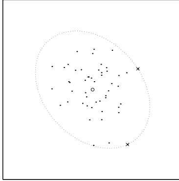
Figure 4: In the dual of the D -optimal experiment design problem we compute the minimum-volume ellipsoid, centered at the origin, that contains the test vectors. The test vectors with a nonzero weight lie on the boundary of the optimal ellipsoid. Same data and notation as in Figure 2.
