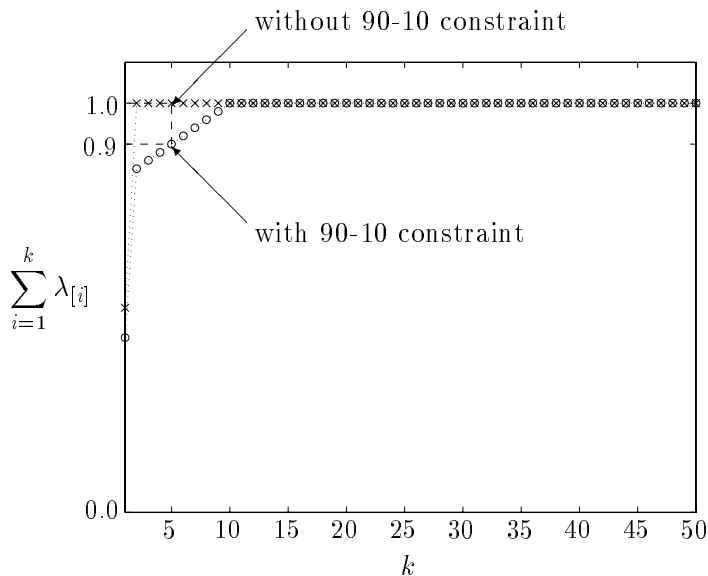
Figure 3: Experiment design of Figure 2. The curves show the sum of the largest k components of \lambda as a function of k , without the 90-10 constraint ('x'), and with the constraint ('o'). The constraint specifies that the sum of the largest five components should be less than 0.9, i.e. , the curve should avoid the area inside the dashed rectangle.
