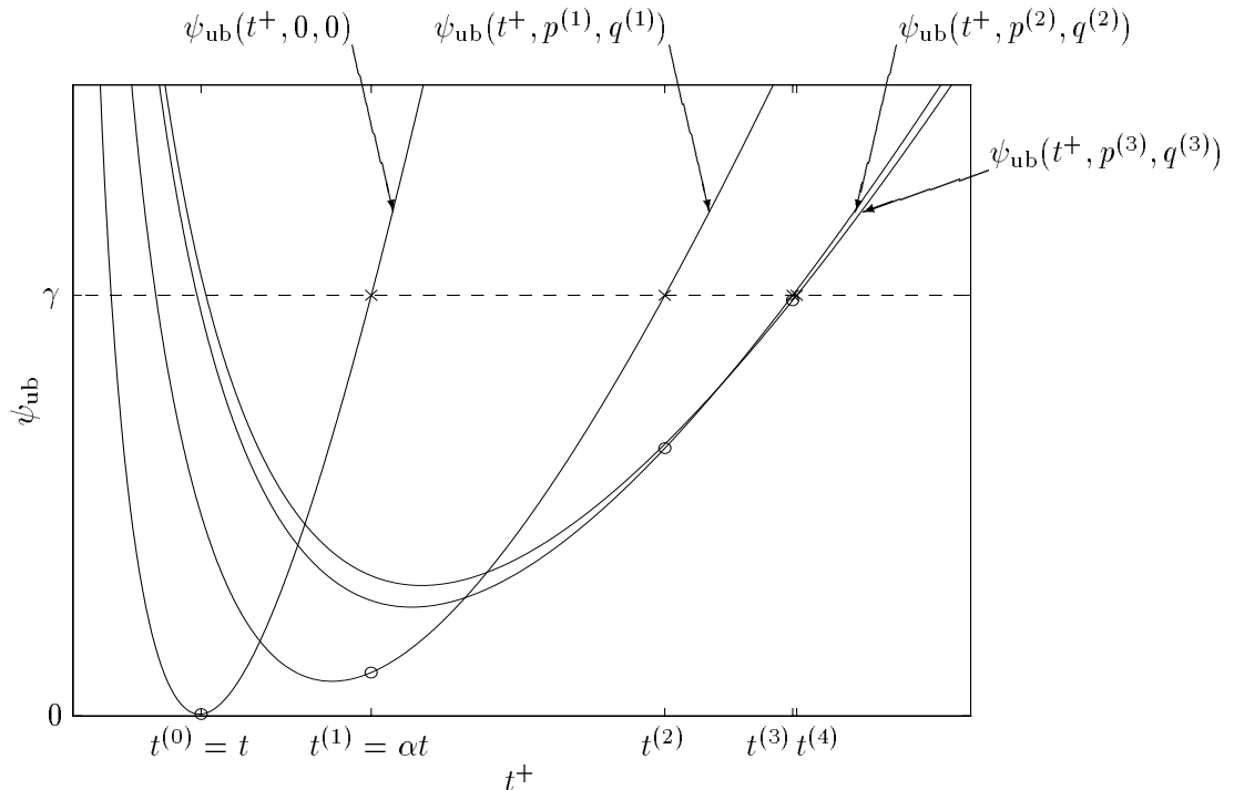
Figure 6: Parameter selection and predictor step in long-step algorithm alternates between minimizing \psi_{\text{ub}}(t^+, p, q) over primal step length p and dual step length q , and then increasing t^+ until \psi_{\text{ub}}(t^+, p, q) = \gamma .
