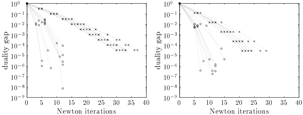
Figure 7: Duality gap versus number of Newton steps for randomly generated maxdet-problems of dimension l = 10 , n = 10 , m = 10 . Left: \gamma = 10 . Right: \gamma = 50 . The crosses are the results for the fixed-reduction method; the circles are the results for the long-step method. Every cross/circle represents the gap at the end of an outer iteration.
