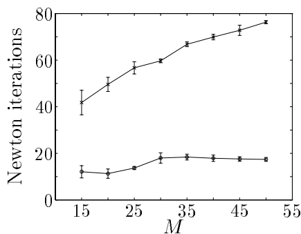
Figure 9: Newton iterations versus problem size for family of experiment design problems of §2.6 including 90-10 rule. Fixed reduction method (top curve) and long-step method (lower curve). \gamma = 10 , p = 10 , M = 15-50 . The curves show the average over 10 problem instances. The error bars indicate the standard deviation.
