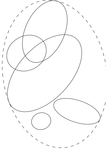
Figure 1: Minimum volume ellipsoid containing five given ellipsoids. Finding such an ellipsoid can be cast as a maxdet-problem, hence efficiently solved.
