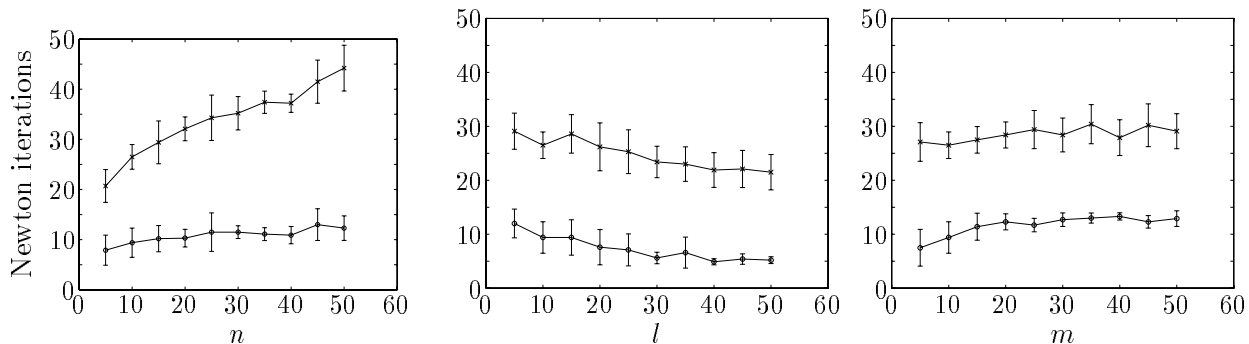
Figure 8: Newton iterations versus problem size for family of random problems. Fixed reduction method (top curve) and long-step method (lower curve). \gamma = 10 . Left. l = 10 , n = 5-50 , m = 10 . Middle. l = 5-50 , n = 10 , m = 10 . Right. l = 10 , n = 10 , m = 5-50 . The curves give the average over 10 problem instances. The error bars indicate the standard deviation.
