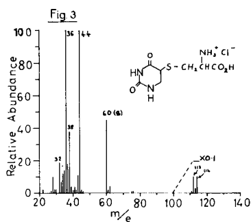
FIGURE 3: Mass spectrum of the heterodimer of uracil and cysteine as the hydrochloride. An Associated Electrical Industries MS9 mass spectrometer was used. The source temperature was 230°.
